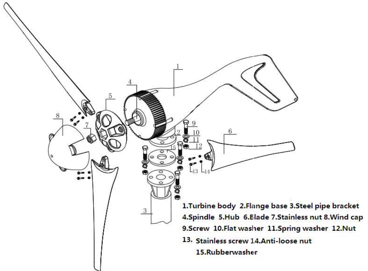
Figure 3 wind turbine decomposition
